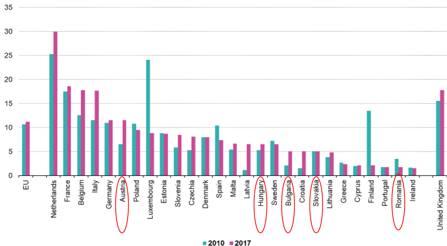
Circular material use rate in 2010 and 2017
